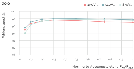
Fronius Verto 30.0
